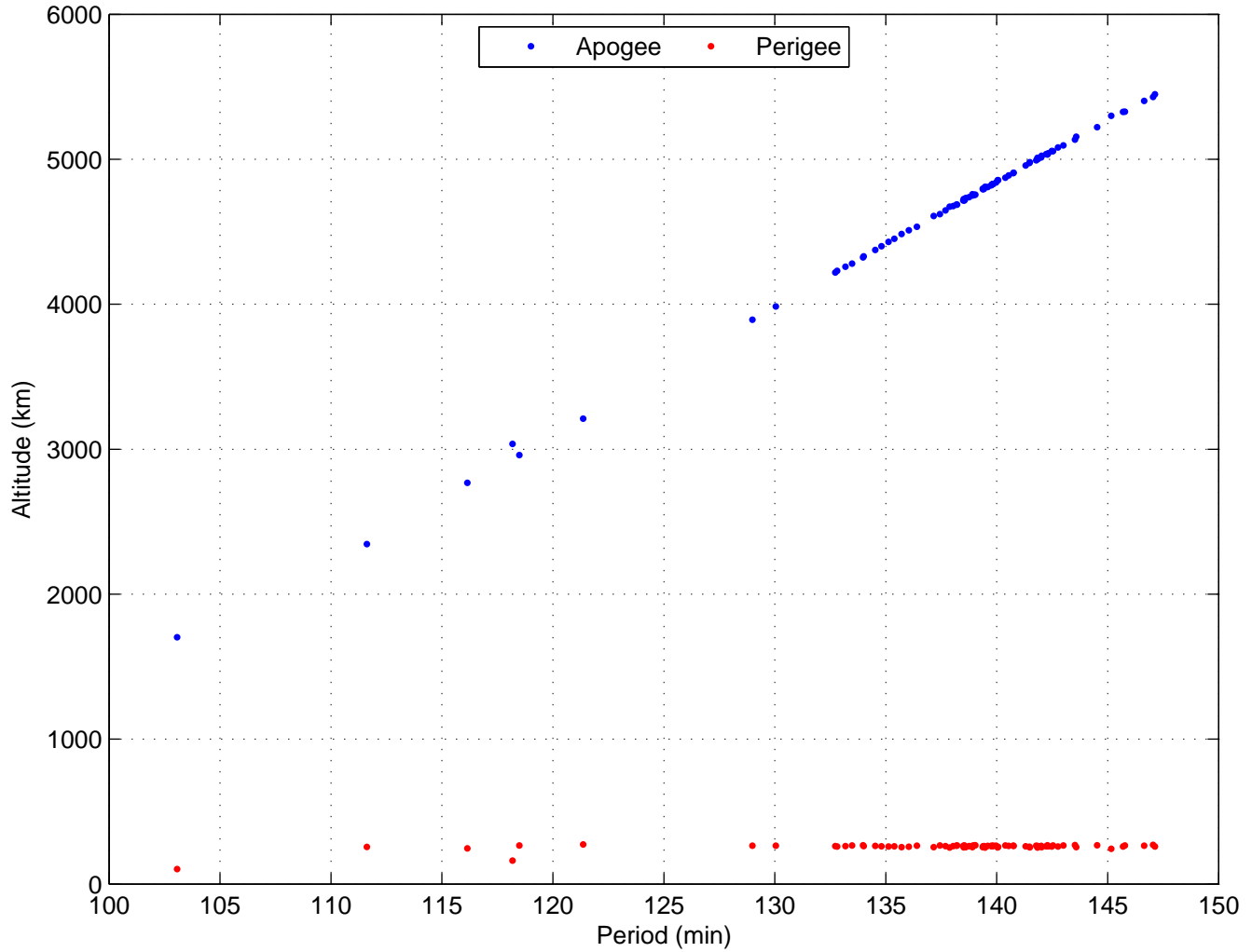
Gabbard Plot of Breeze-M Rocket Body (38746) Breakup (81 pieces)
